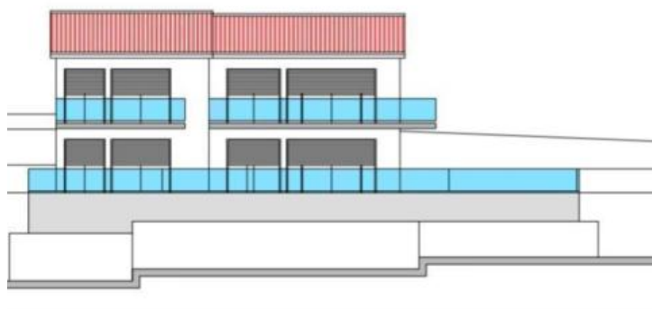
FRONT FACAD 1:100
